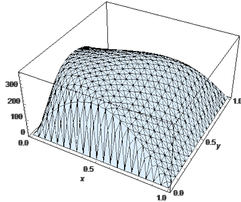
Fig. 3. Graph of the approximation u_h|_K \in P_1(K) , n = 2
