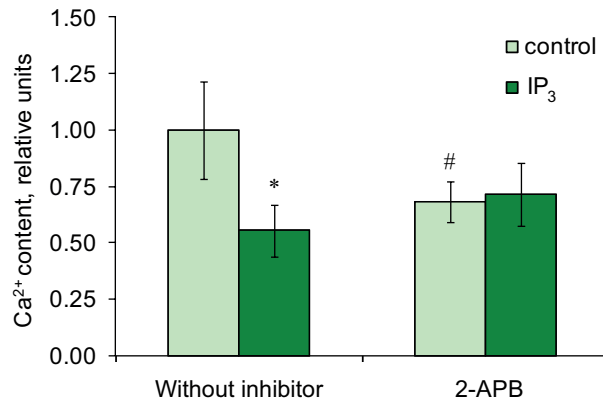
Fig. 1. The effect of IP 3 on Ca 2+ content in the permeabilized secretory cells of rat exorbital lacrimal gland: tissue Ca 2+ content in the absence of inhibitors/agonists was normalized to one; incubation time – 15 min; [K + ] = 140 mM, [Ca 2+ ] = 10 -7 M; [IP 3 ] = 2 μM; [2-APB] = 10 μM; * – the difference compared with the control reliable with P < 0.05; # – difference compared with the sample without inhibitor/agonist significant with P < 0.05; n = 6 [36]
