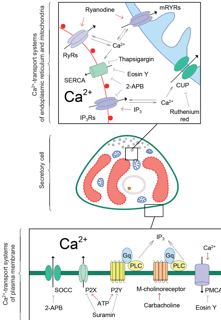
Fig. 7. Scheme of coordinated functioning of different \text{Ca}^{2+} -transport systems in extraorbital lacrimal gland cells of the rat:
